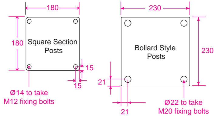
Base Plate Footprints
